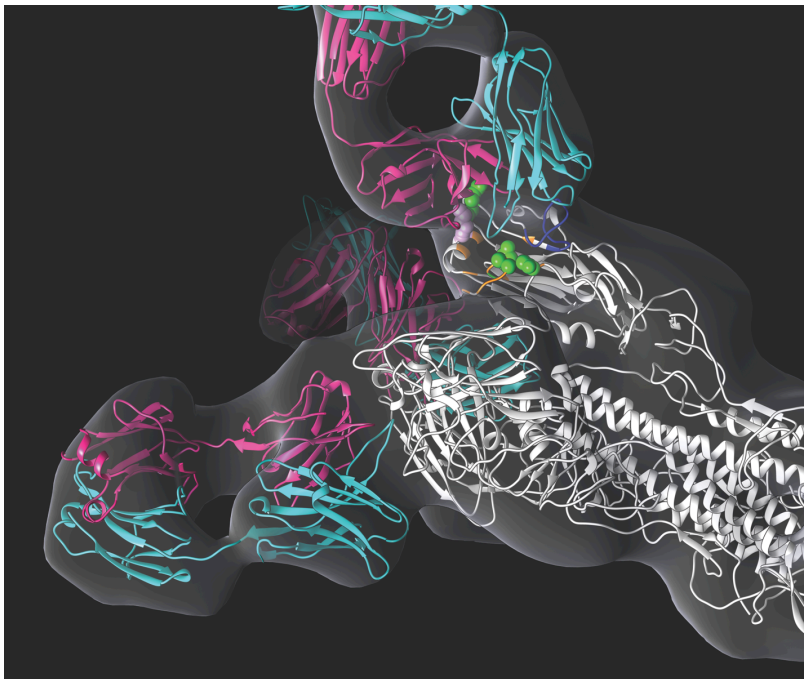
Human monoclonal antibody on influenza H5 HA
